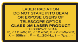
Laser warning sign and laser label LLT30xx-200
