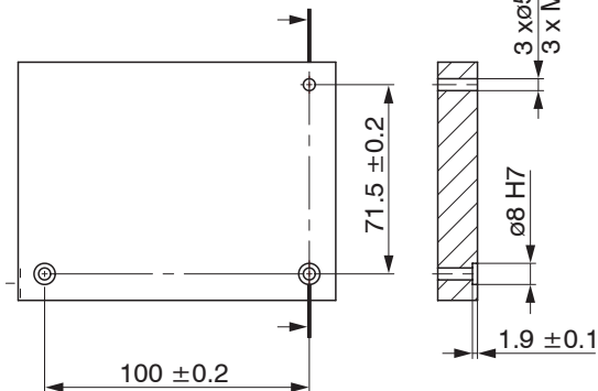
Fig. 6 Dimensional drawing mounting bores, dimensions in mm (inches, rounded off)
