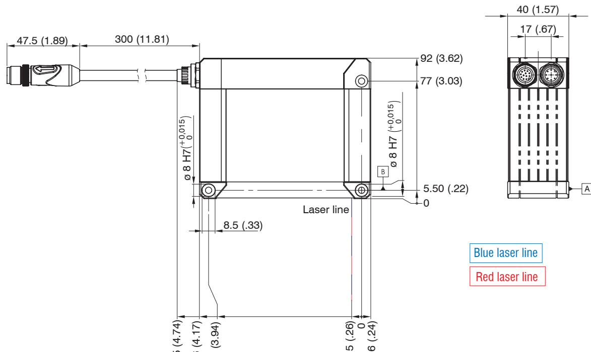
Fig. 19 Dimensional drawing sensor scanCONTROL option RT for LLT30xx-25 / LLT30xx-50 / LLT30xx-100 / LLT30xx-200, dimensions in mm (inches, rounded off)
