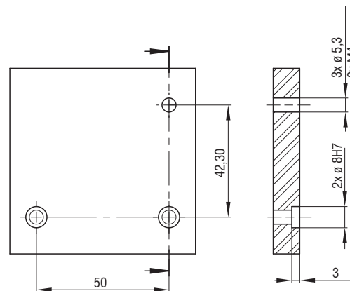
Fig. 8 Dimensional drawing mounting bores, dimensions in mm (inches, rounded off)
