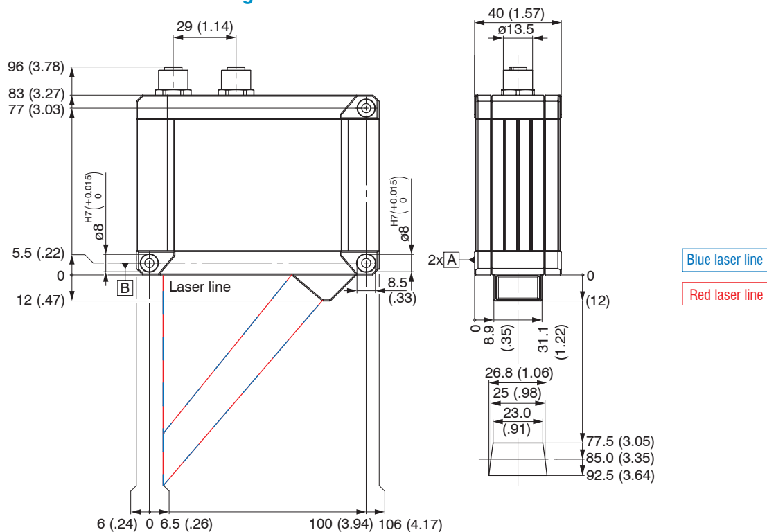
Fig. 15 Dimensional drawing sensor scanCONTROL 30xx-25, dimensions in mm (inches, rounded off)
