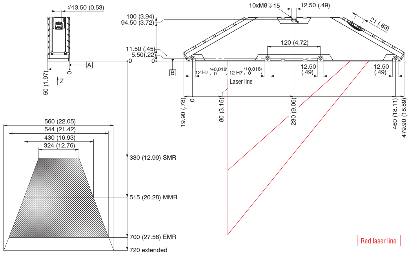
Fig. 20 Dimensional drawing sensor scanCONTROL 30xx-430, dimensions in mm (inches, rounded off)
