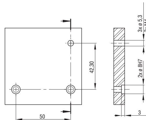
Fig. 10 Dimensional drawing mounting bores, dimensions in mm (inches, rounded off)
