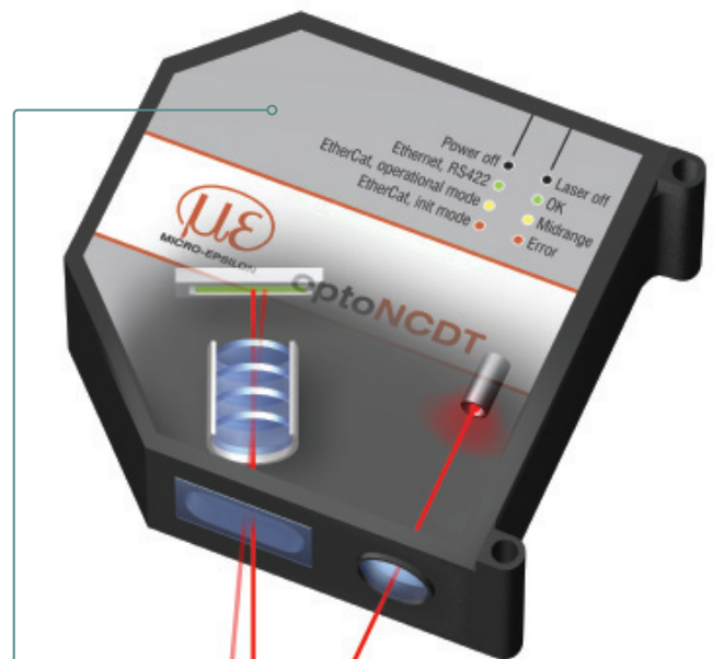
The non-contact displacement sensors optoNCDT utilize optical triangulation as a general measuring principle
