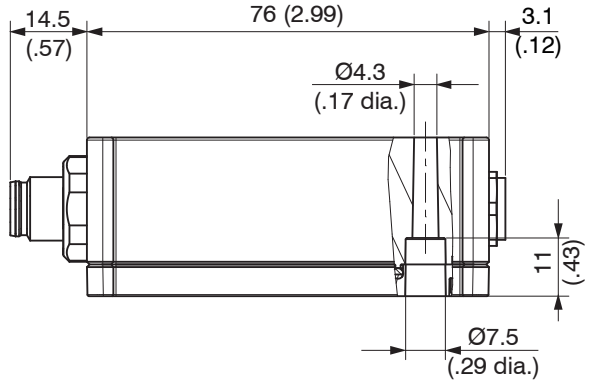
Fig. 5 Dimensional drawing of MSC7401(010) controller, dimensions in mm (inches)
